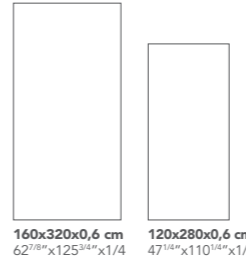
6 mm thick
